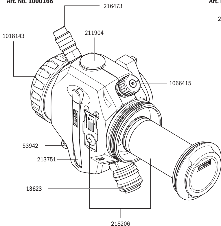
Spare parts for: SATA air carbon regulator Art. No. 1000166
