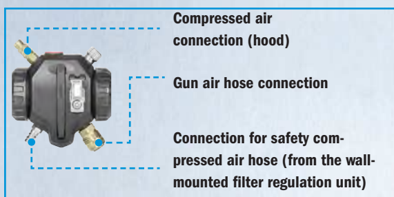
Accessories: SATA air humidifier Art. No. 1000299
